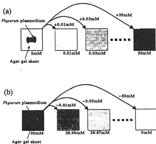
Fig. 1. Regulation procedure of chemical environment around the plasmodium. (a) Concentration increase. (b) Concentration decrease.
